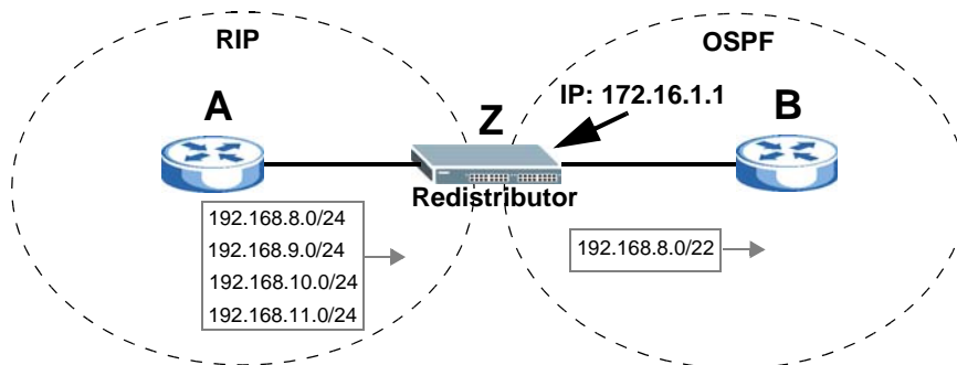
Figure 9 OSPF Redistribution Summary Address Example
