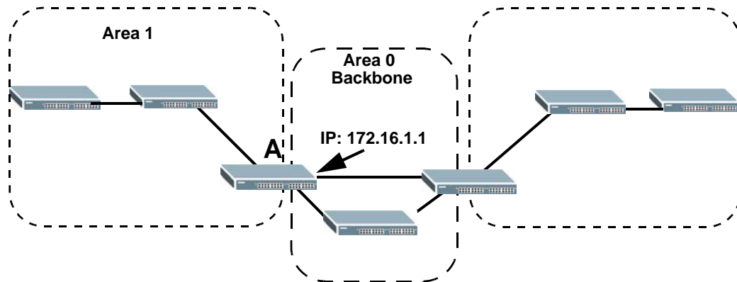
Figure 8 OSPF Network Example
