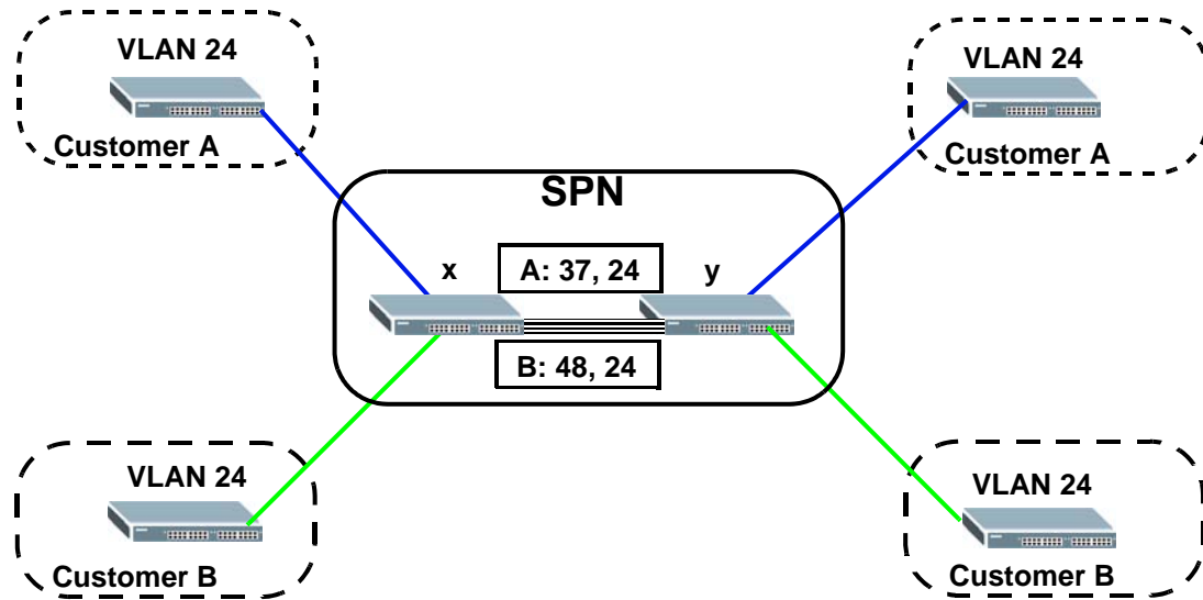
Figure 11 Example: VLAN Stacking
