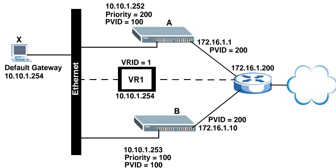
Figure 12 Example: VRRP
