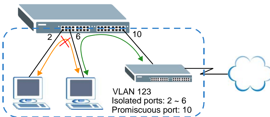
Figure 10 Private VLAN Example
